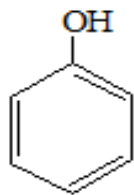
Phenol
