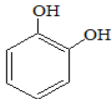
Benzene-1,2-diol C.N : Catechol
