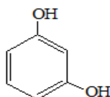
Benzene-1,3-diol C.N : Resorcinol
