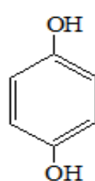
Benzene-1,4-diol C.N : Hydroquinone / quinol
