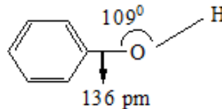
Phenol
