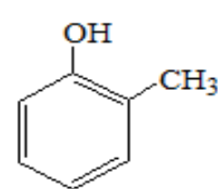
2-Methylphenol C.N : o-Cresol
