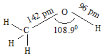
Methanol
