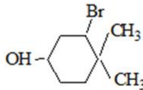
3-Bromo-4,4-dimethylcyclohexanol
