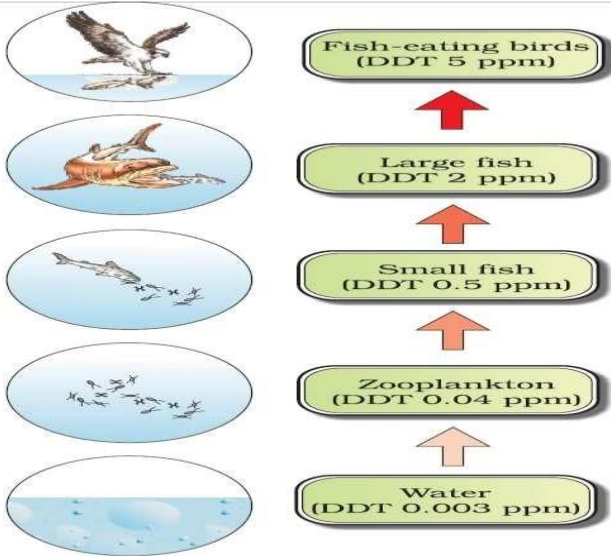
Figure- Biomagnification of DDT in an aquatic food chain
