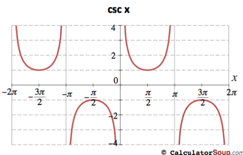
y = \operatorname{cosec} x
