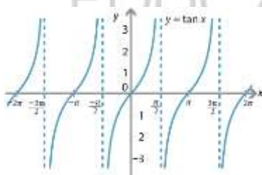
y = \tan x
