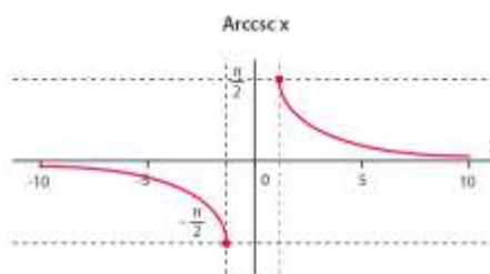
y = \operatorname{cosec}^{-1} x
