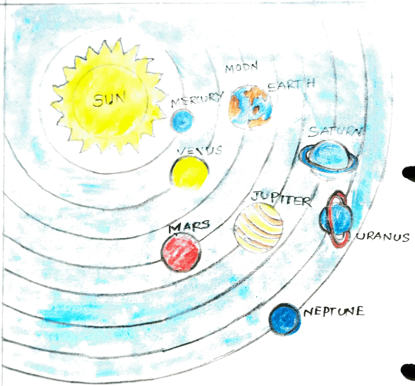
SOLAR SYSTEM
