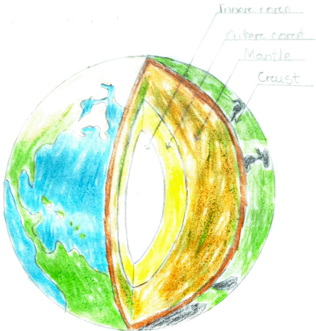
Various Layers of Earth
