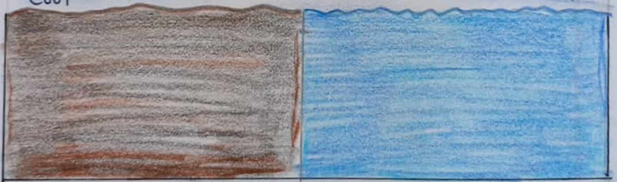
Sea Breeze and Land Breeze
