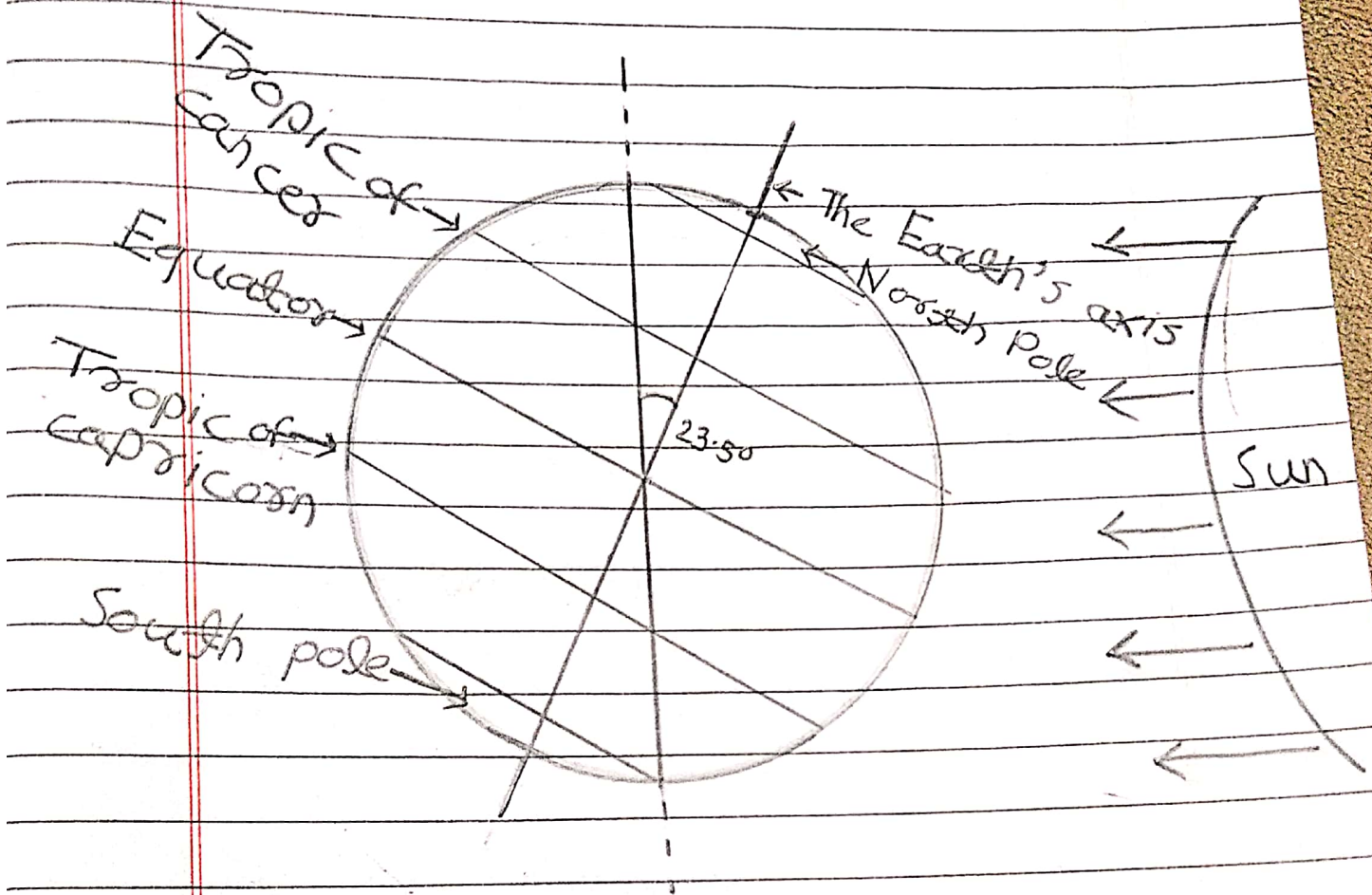
Labelled Diagram of Earth's rotation.
