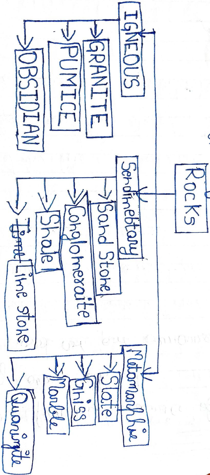
Flowchart of types of rocks
