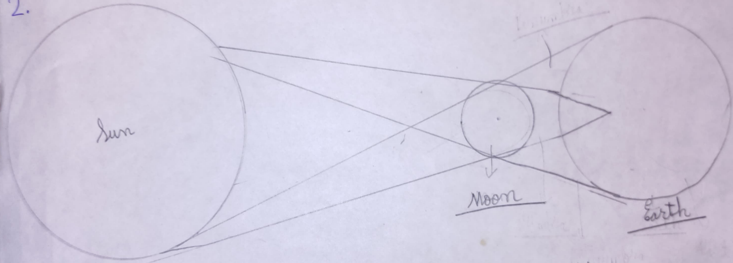
Formation of total solar eclipse
