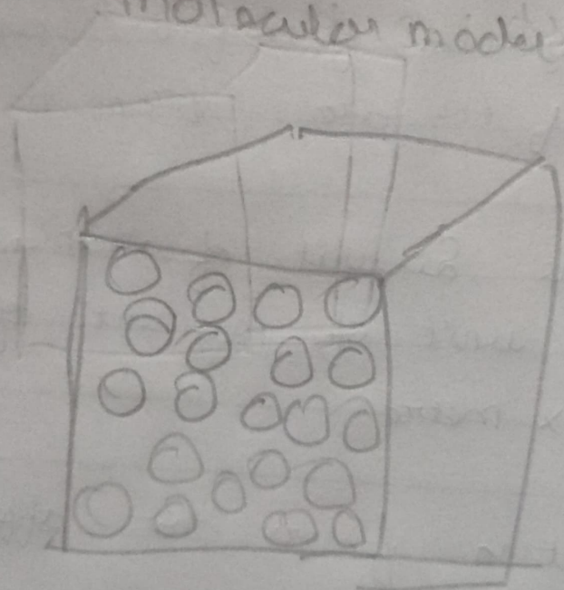
molecular model in liquid
