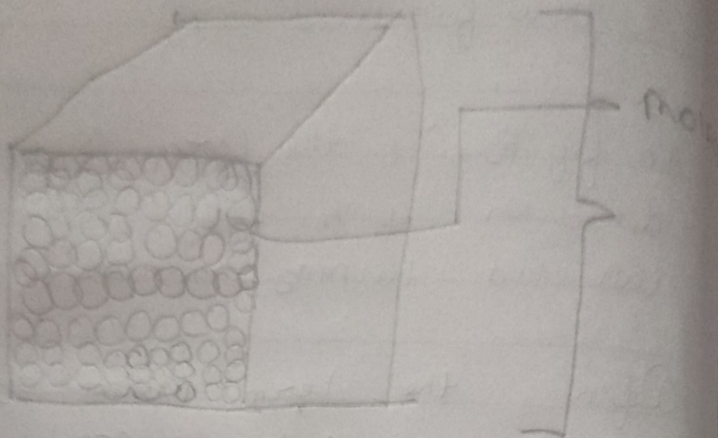
molecular model of solid
