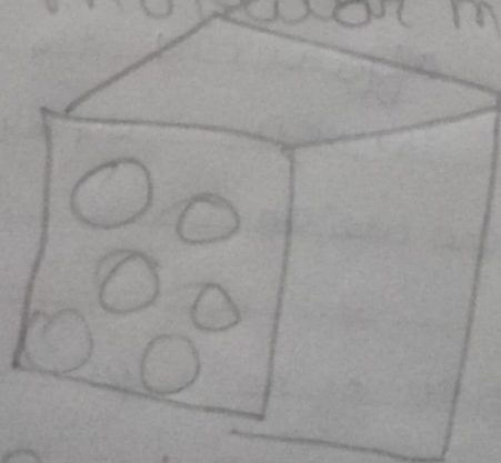
molecular model in gas
